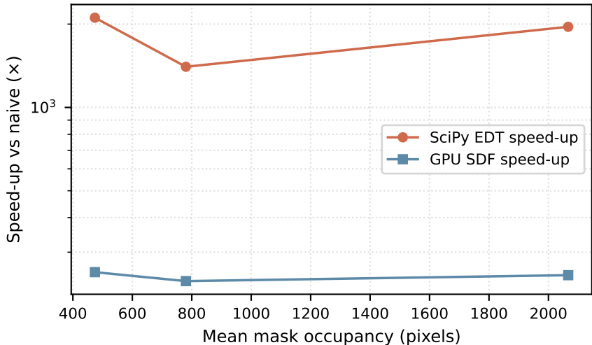
Speed-up vs barrier-mask occupancy
