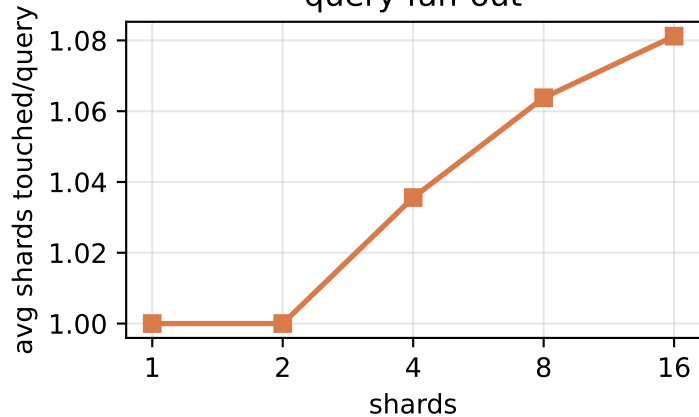
query fan-out
