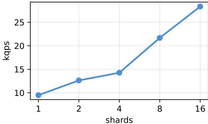
kd-tree shard throughput
