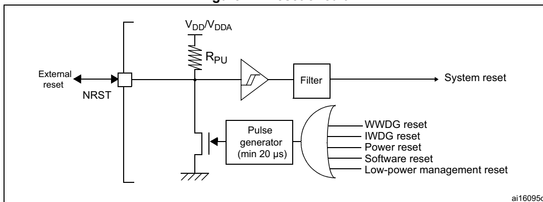
Figure 11. Reset circuit
