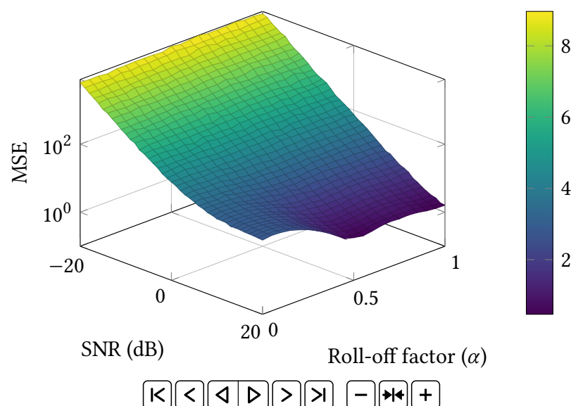
Over-The-Air Computing MSE Profile (sps = 1 \times 10^1 )
