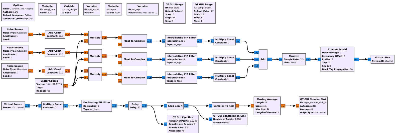
Figure 9: GNU Radio flowgraph for the ideal, Nyquist-compliant scenario.
