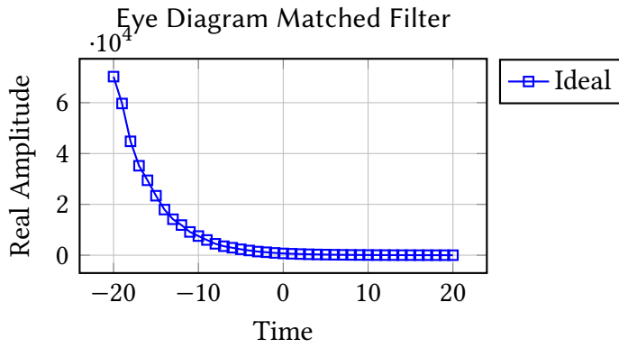
(a) Eye Diagram of the ideal OTA computation network over an AWGN channel.
