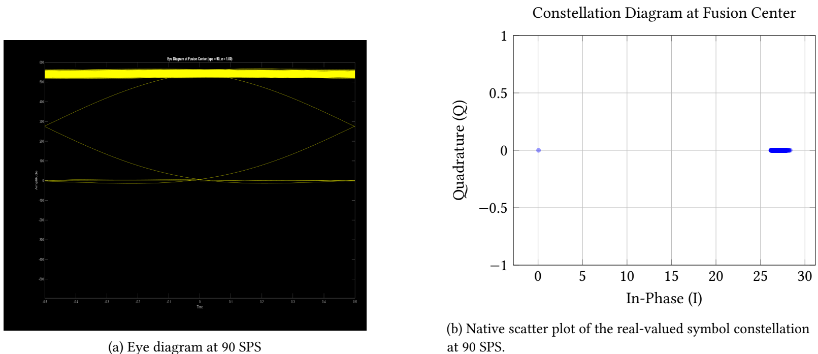
Figure 3: Signal integrity analysis at the Fusion Center. Left: Eye diagram illustrating Inter-Symbol Interference bounds. Right: Native scatter plot of the real-valued symbol constellation.
