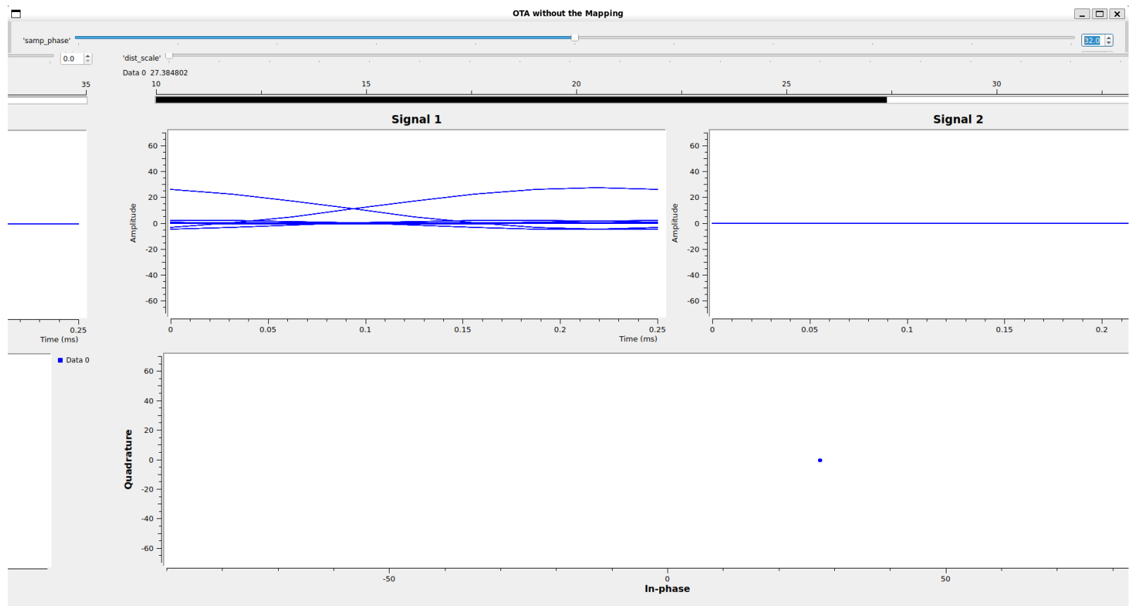
Figure 10: GNU Radio Eye & Constellation Diagram for the ideal, Nyquist-compliant scenario.
