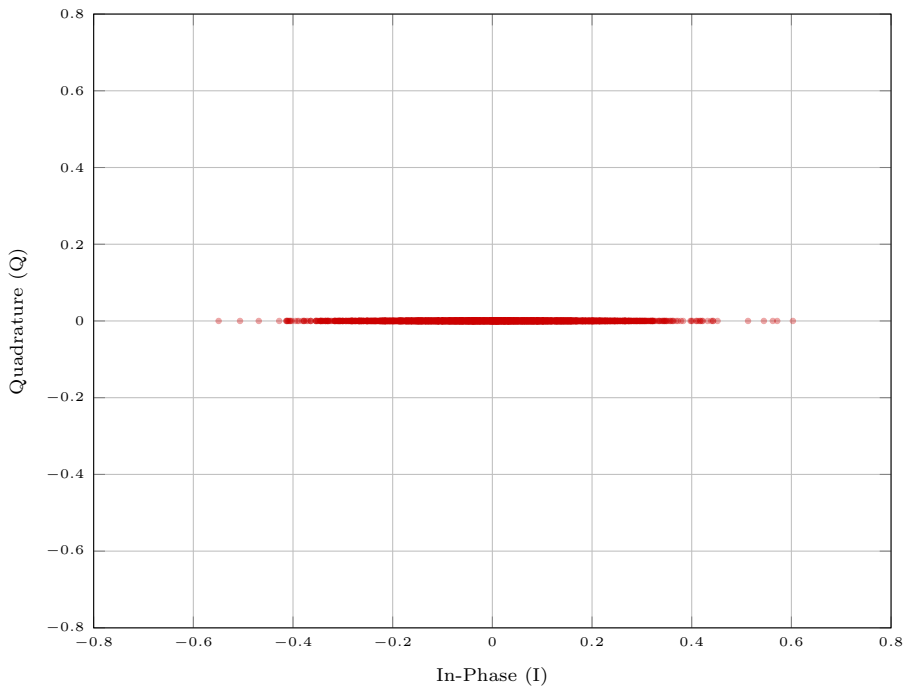
Asynchronous AirComp Constellation ( \alpha = 0.70 , SNR = 20 dB)
