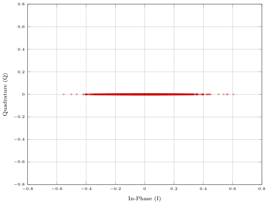
Asynchronous AirComp Constellation ( \alpha = 0.90 , SNR = 20 dB)
