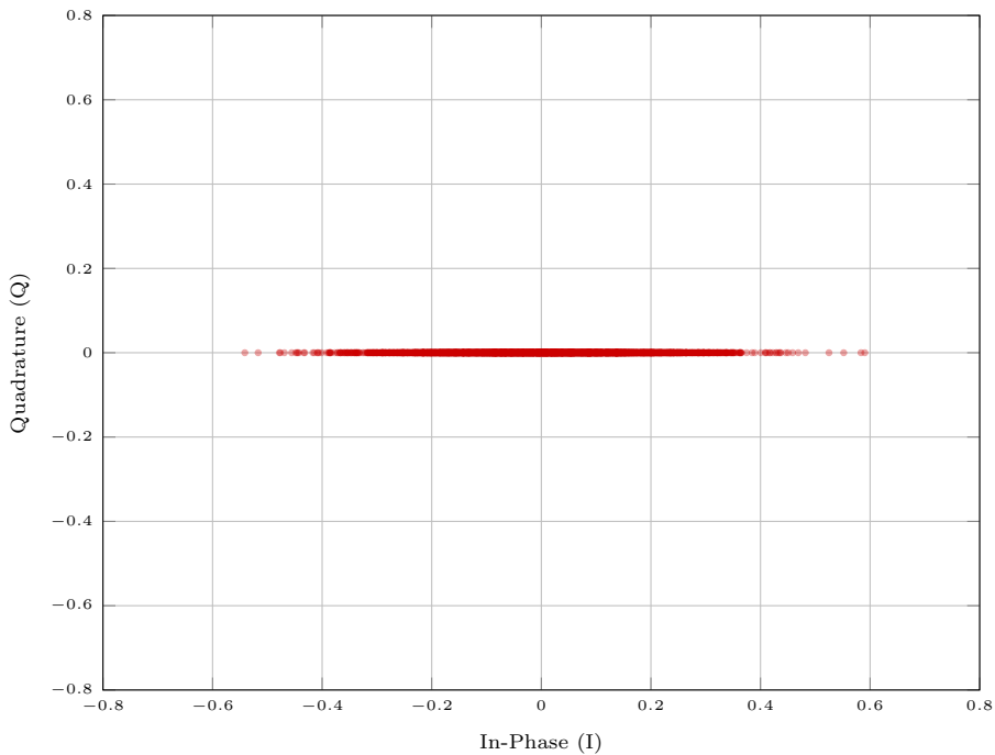
Asynchronous AirComp Constellation ( \alpha = 0.00 , SNR = 20 dB)
