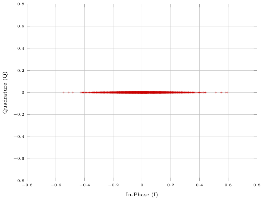
Asynchronous AirComp Constellation ( \alpha = 0.80 , SNR = 20 dB)
