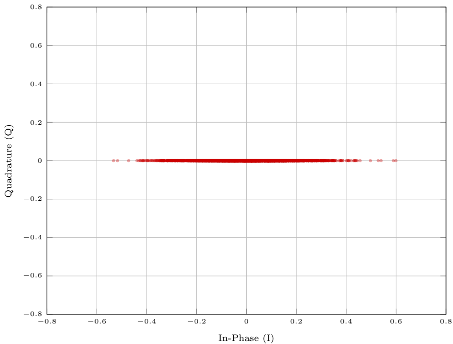
Asynchronous AirComp Constellation ( \alpha = 0.20 , SNR = 20 dB)
