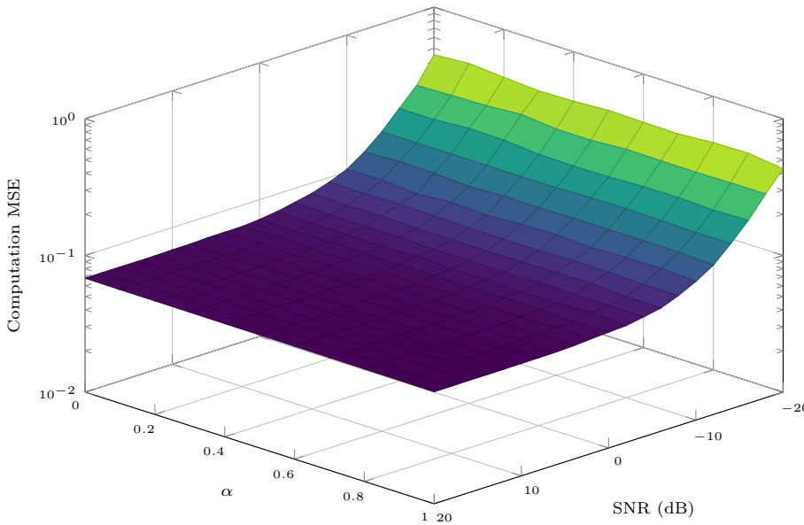
Asynchronous AirComp with CFO ( sps = 12 )
