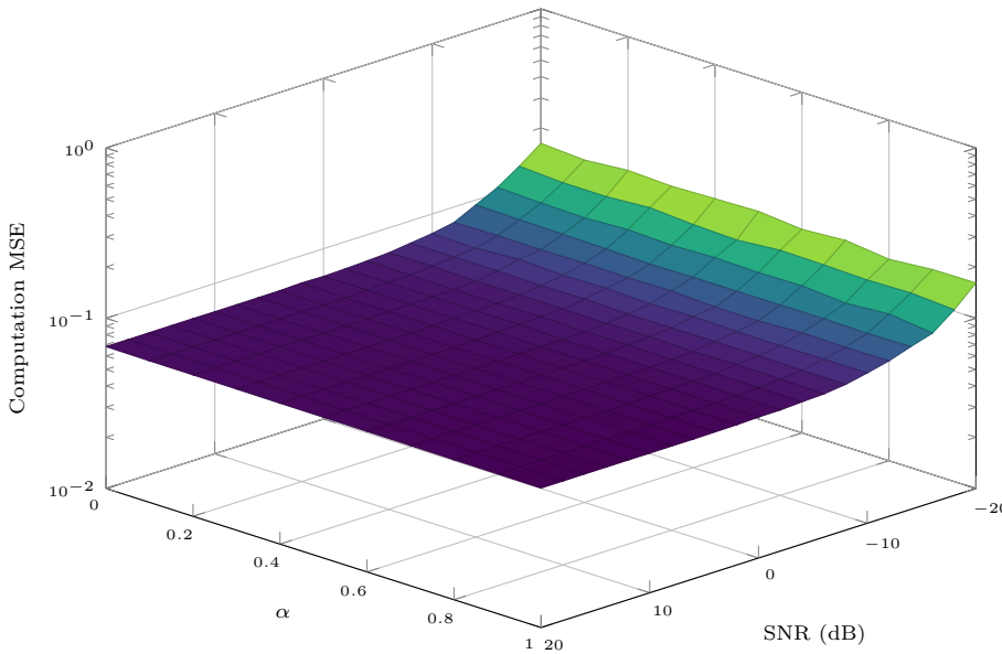
Asynchronous AirComp with CFO ( sps = 48 )
