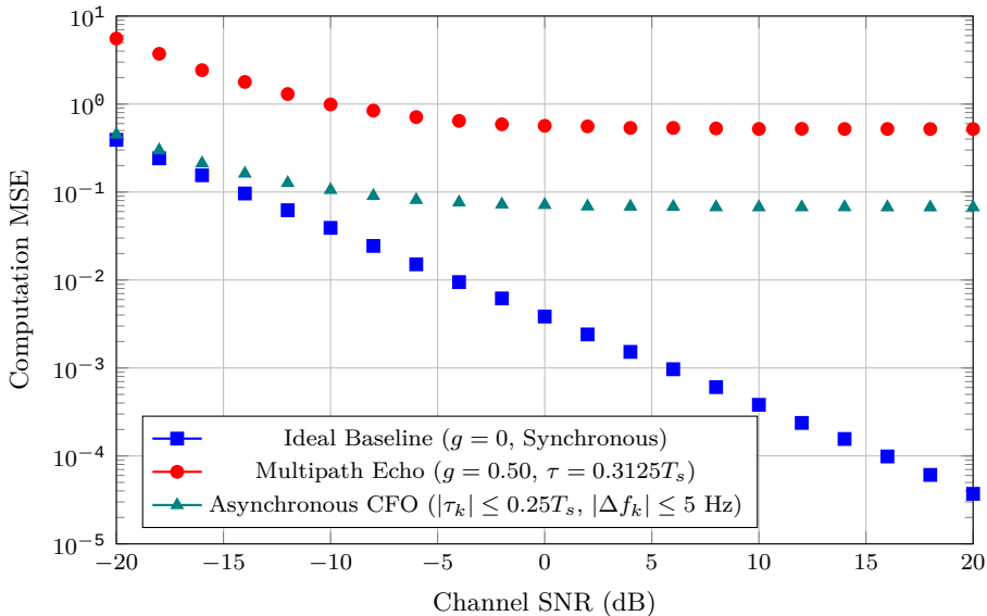
AirComp MSE across Channel Impairment Regimes (SPS = 12, \alpha = 0.50 )
