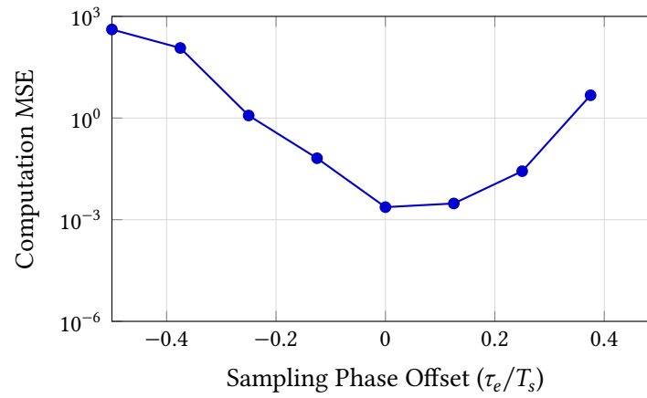
Figure 8: S-Curve of OTA computation to symbol timing synchronization error (sps = 8).
