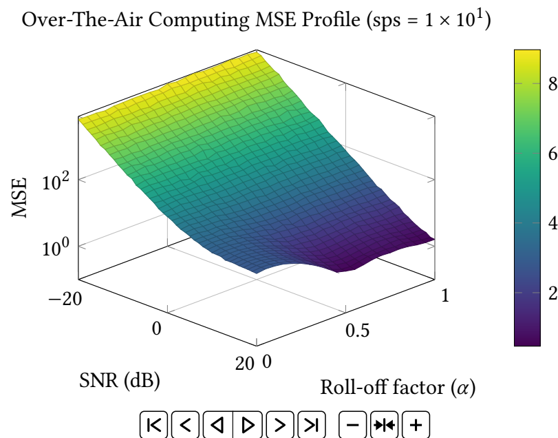
Figure 2: Interactive OTA computing animation demonstrating the architectural impact of Samples Per Symbol ( \text{sps} ) scaling.
