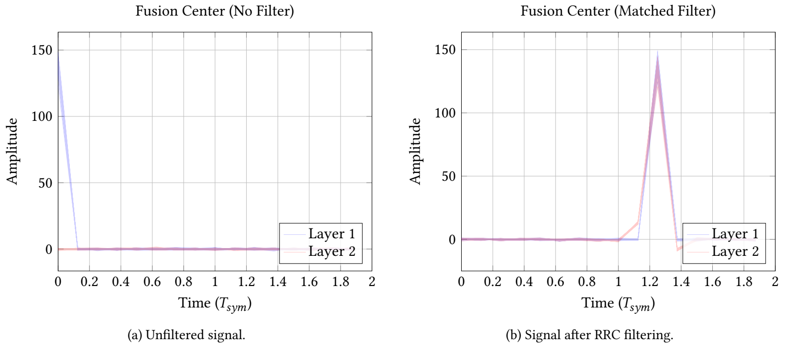
Figure 8: Comparative eye diagrams demonstrating the signal reconstruction at the fusion center.
