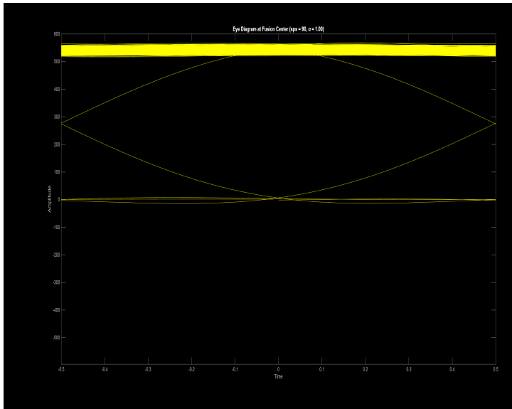
(a) Eye diagram at 90 SPS
