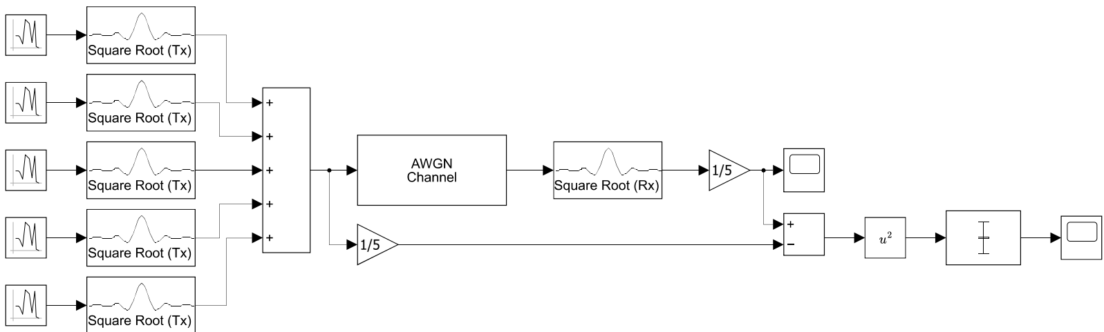
Figure 4: Simulink block diagram representing the ideal OTA computation network over an AWGN channel.
