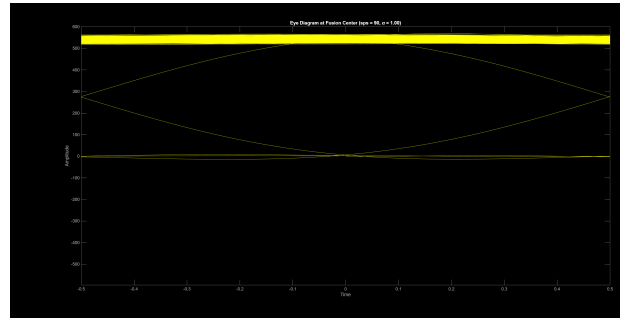
(a) Eye diagram at 90 SPS
