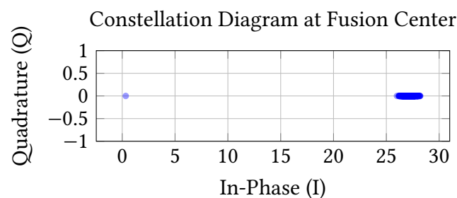
(b) Native scatter plot of the real-valued symbol constellation at 90 SPS.
