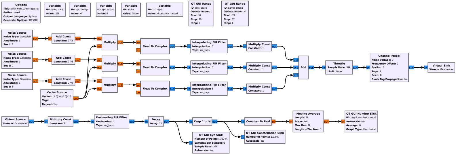
Figure 6: GNU Radio flowgraph for the ideal, Nyquist-compliant scenario.
