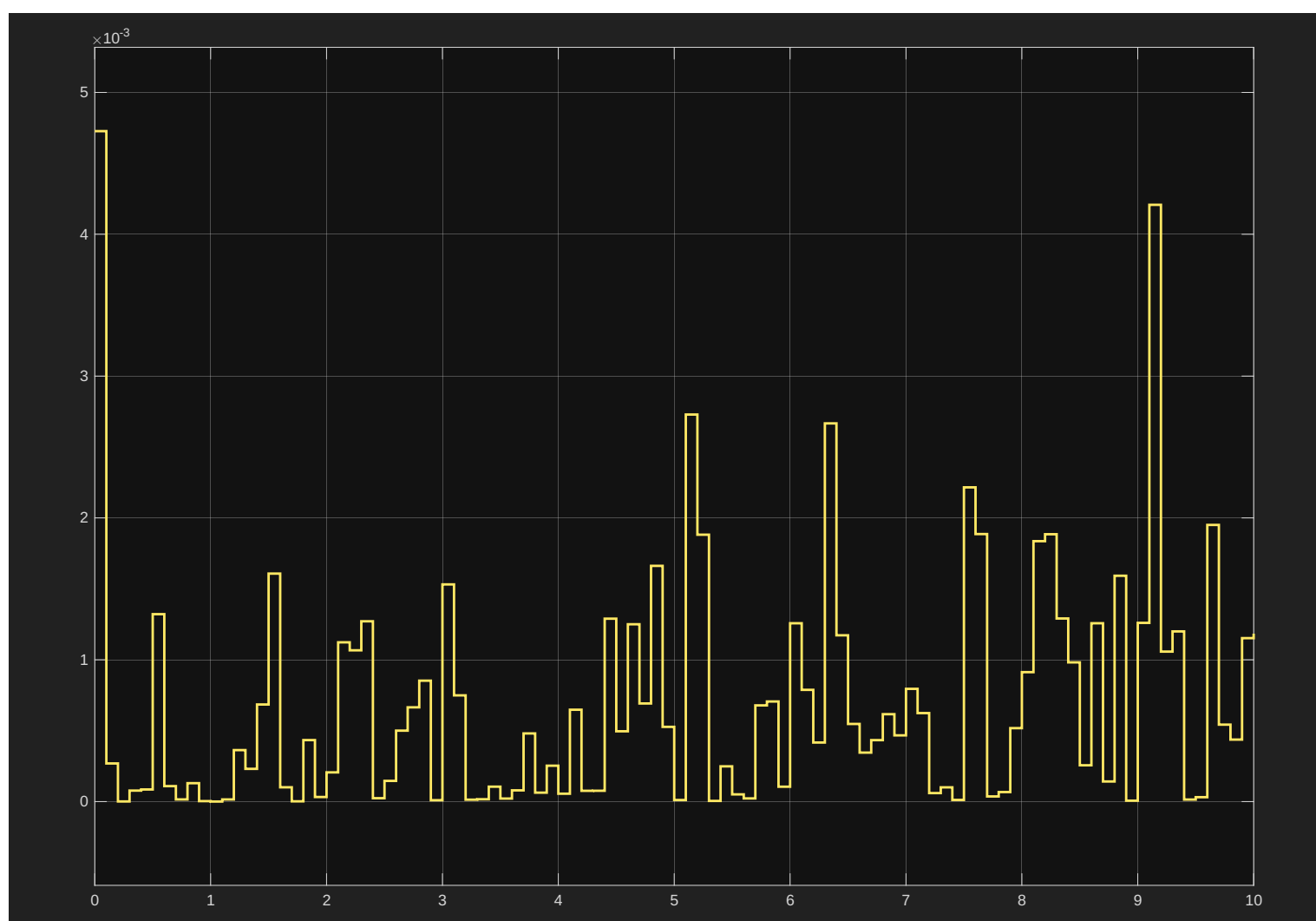
Figure 2: Mean Square Error of the ideal OTA computation network over an AWGN channel.
