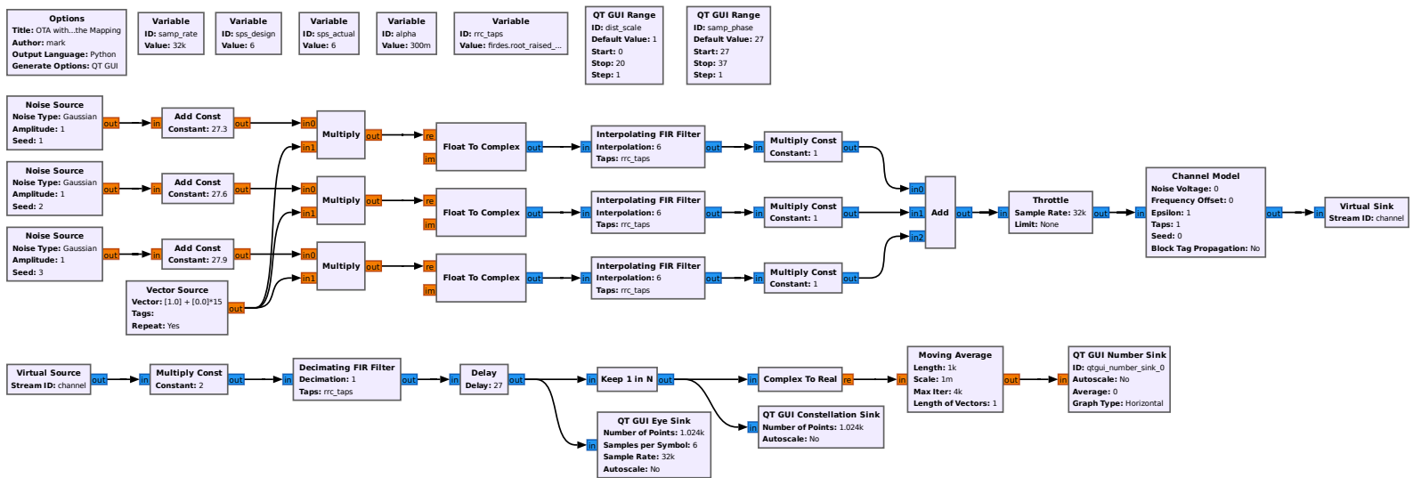
Figure 3: GNU Radio flowgraph for the ideal, Nyquist-compliant scenario.
