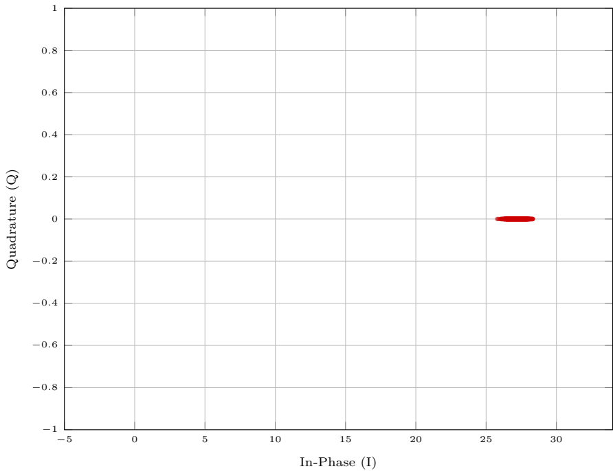
Matched RRC ( \alpha = 0.30 , SNR = 20 dB)
