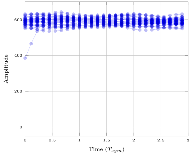
Span = 12 ( sps = 9 )
