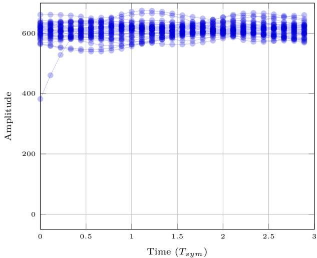
Span = 4 ( sps = 9 )
