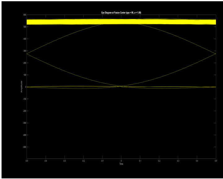
(a) Eye diagram at 90 SPS
