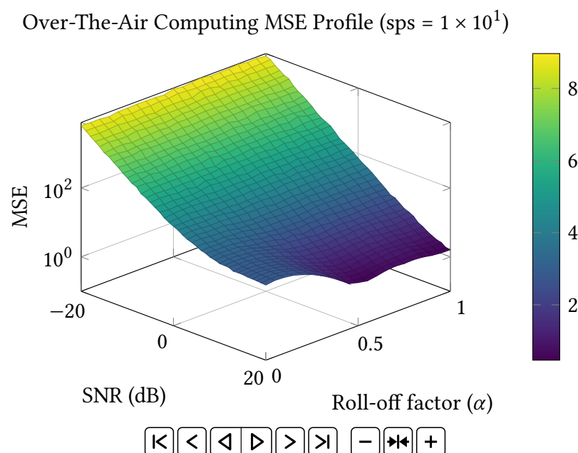
Figure 2: Interactive OTA computing animation demonstrating the architectural impact of Samples Per Symbol ( sps ) scaling.
