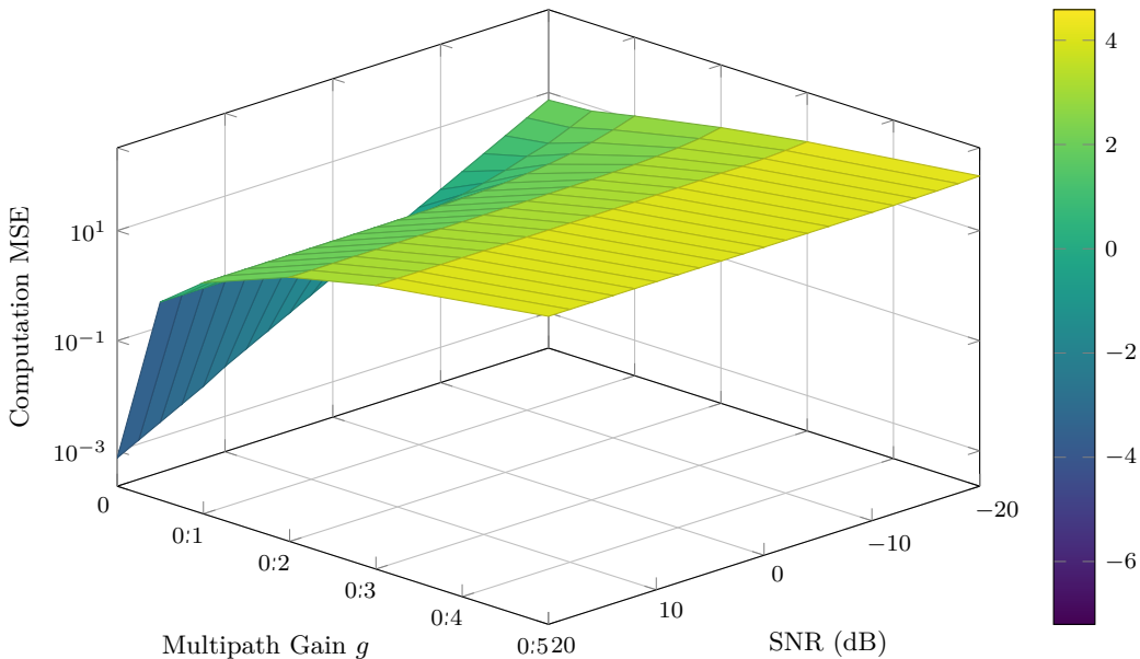
Simulink AirComp MSE Surface vs. SNR and Echo Gain g (SPS = 12)
