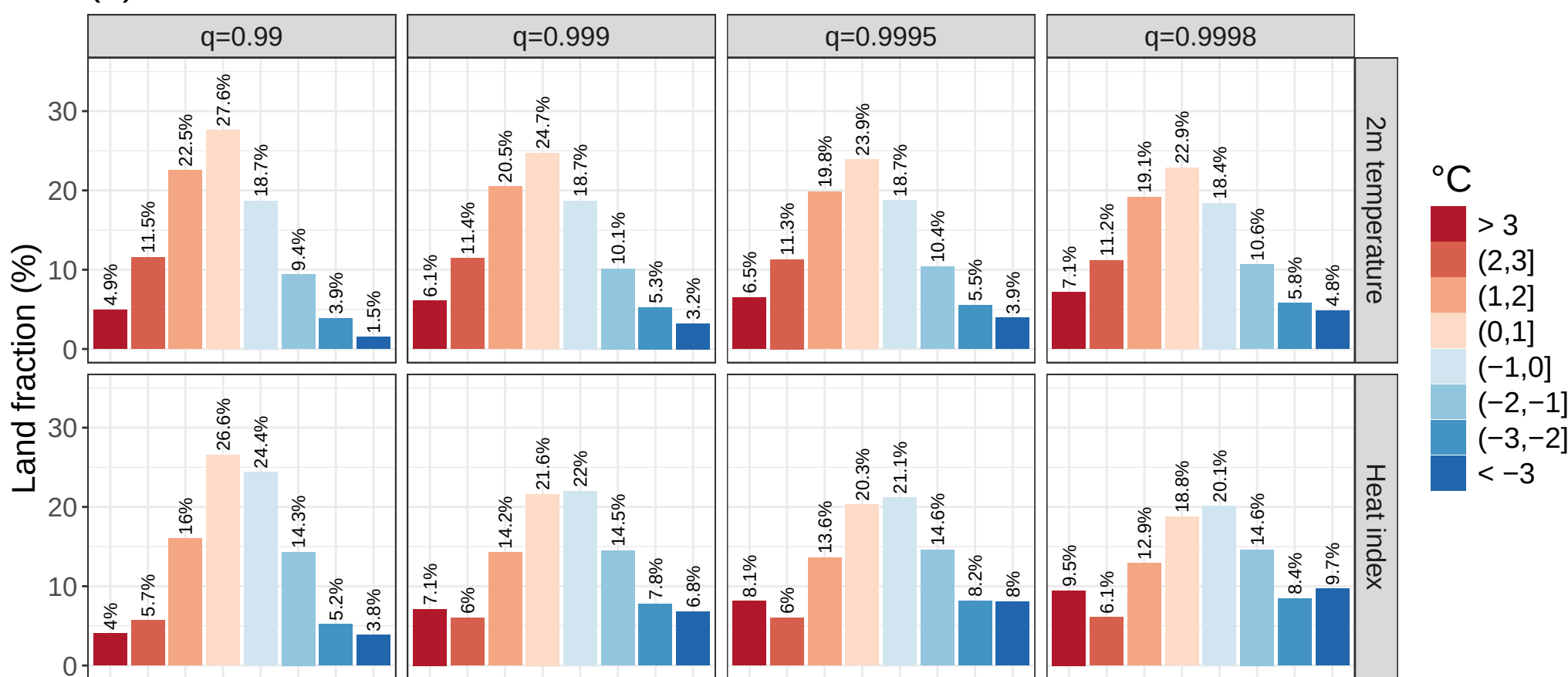
(b) Differences: IFS–GEV minus HENS
