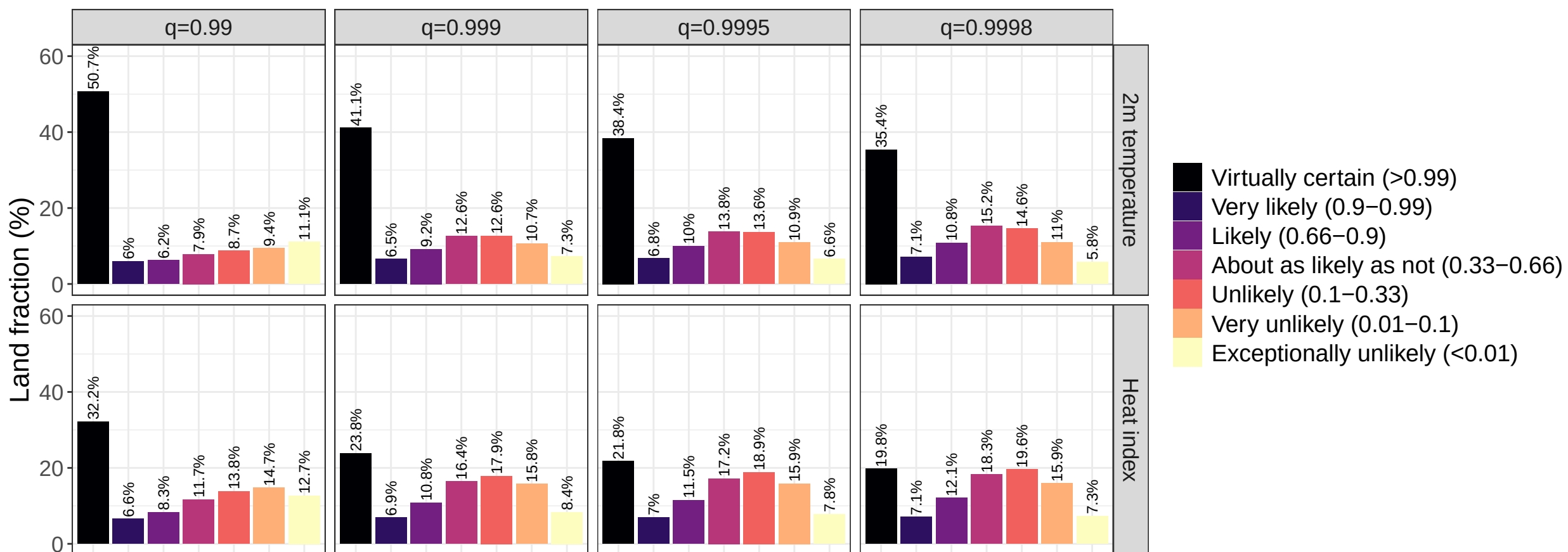
(a) Probability: IFS–GEV contains HENS
