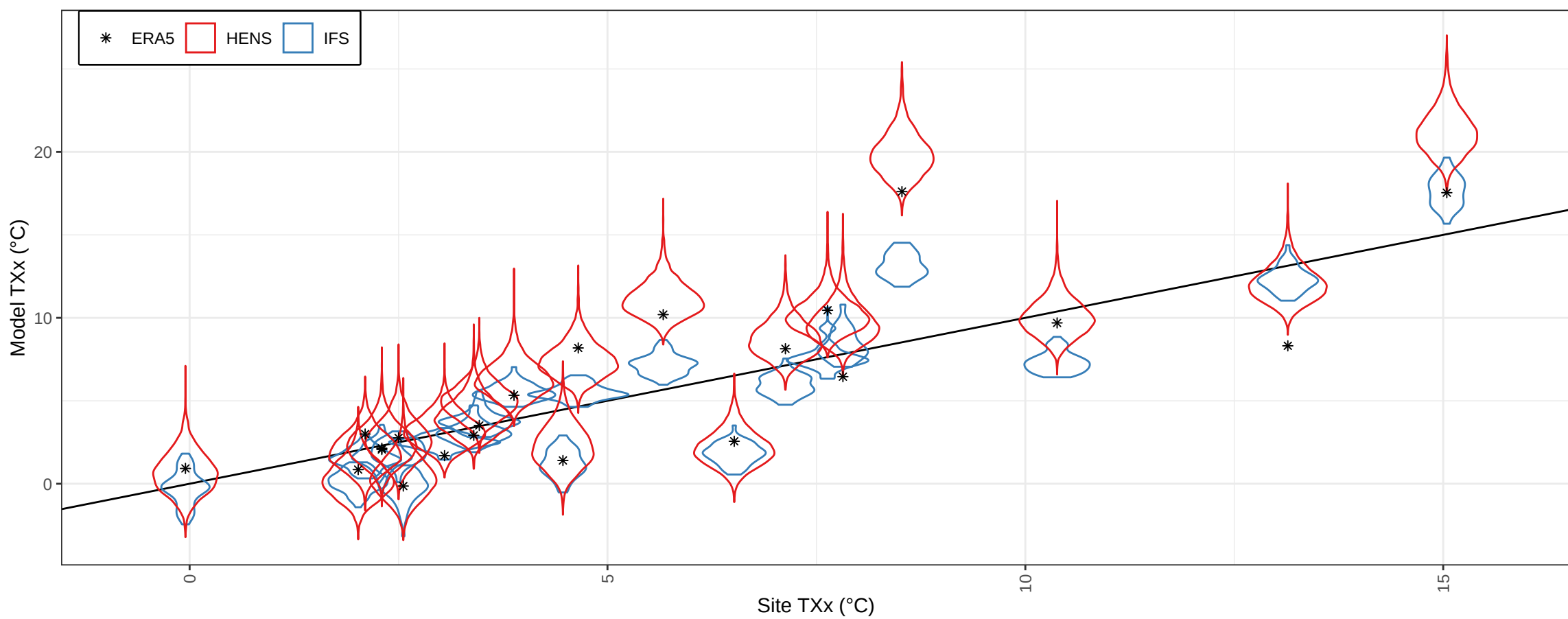
(b) Comparison of station data vs. HENS: all-time TXx
