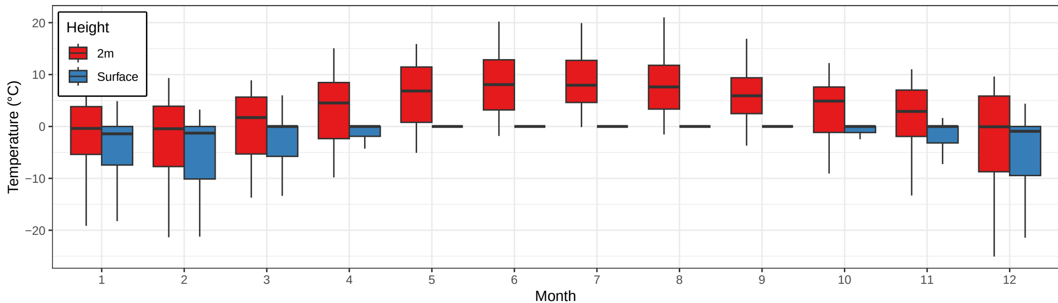
(b) Maximum hourly 2m air temperature
