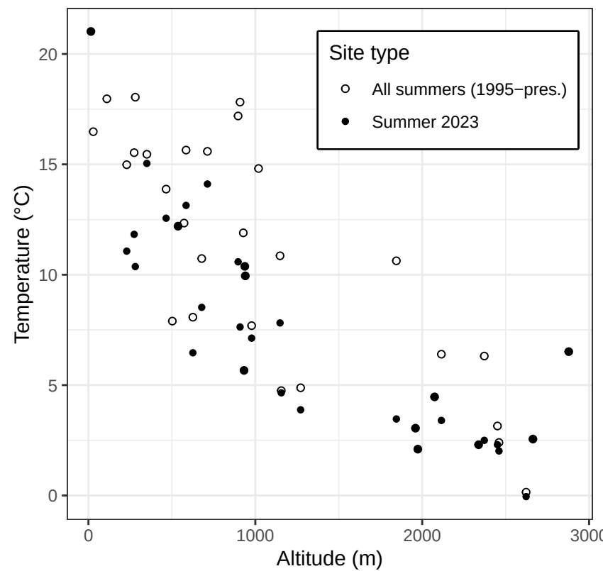
(c) Maxima versus altitude
