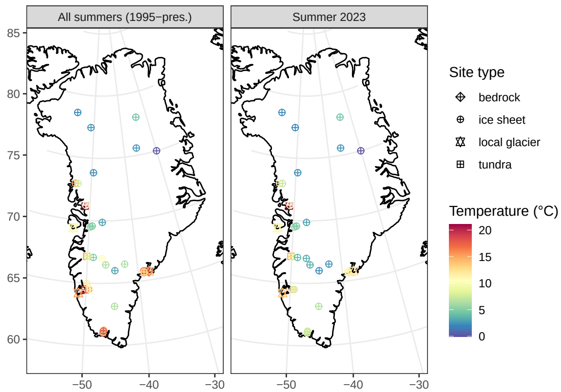
(b) Maximum hourly 2m air temperature
