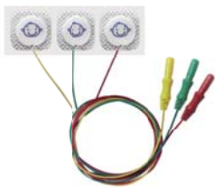
SG15 | Socket \Phi 1.5 Electrode 22mm Y.G.R Lead-wire 60cm
