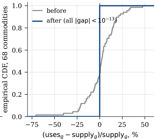
cumulative distribution
