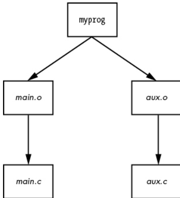
Figure 15-1: Makefile dependencies
