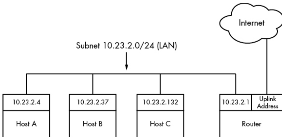
Figure 9-2: Network with IP addresses
