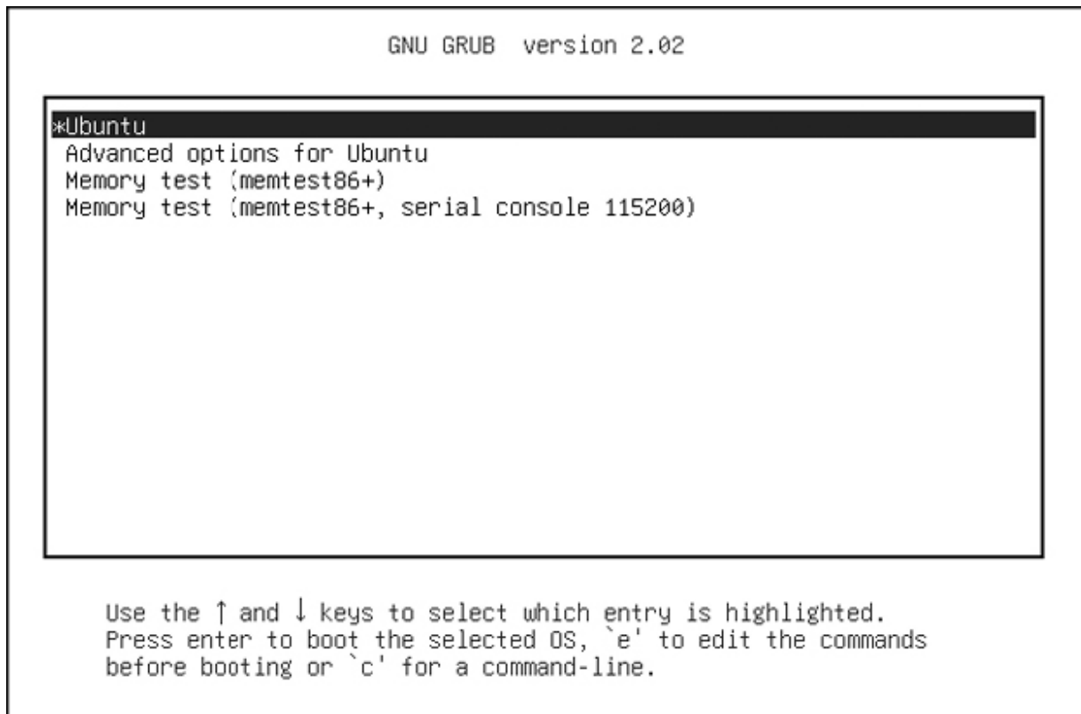
Figure 5-1: GRUB menu
