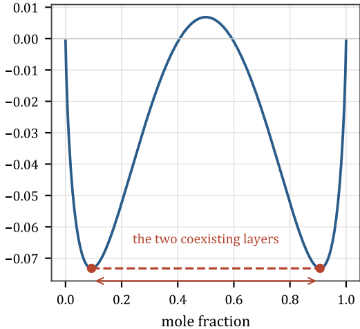
A = 2.8 RT : two liquids
