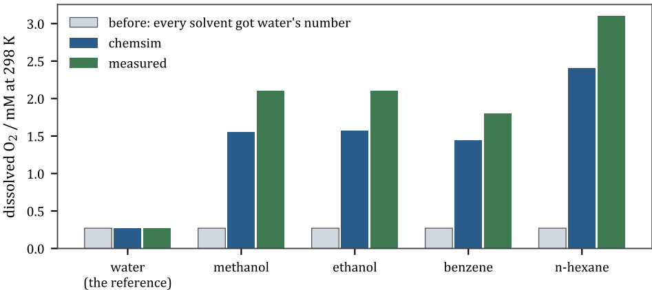
One tabulated constant, transferred to four solvents by \gamma^\infty
