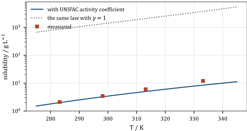
Benzoic acid in water. The ideal law is two to three orders out
