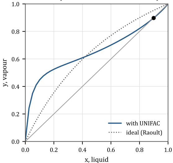
The azeotrope is where this curve crosses y = x
