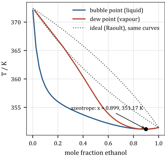
T-x-y, ethanol + water at 1 atm
