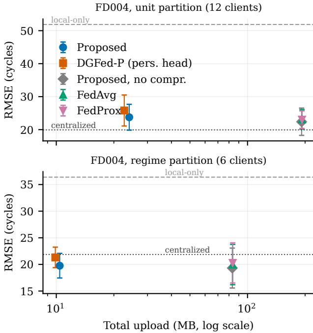
Fig. 2. Communication-accuracy plane on FD004 (both partitions). Total upload (MB, log scale) versus RMSE (mean \pm std) for DGFed, DGFed-P, the no-compression arm, FedAvg, and FedProx; the centralized bound (dotted) and local-only baseline (dashed) are horizontal references. DGFed sits at FedAvg-level accuracy at 8.0\times lower uplink.
