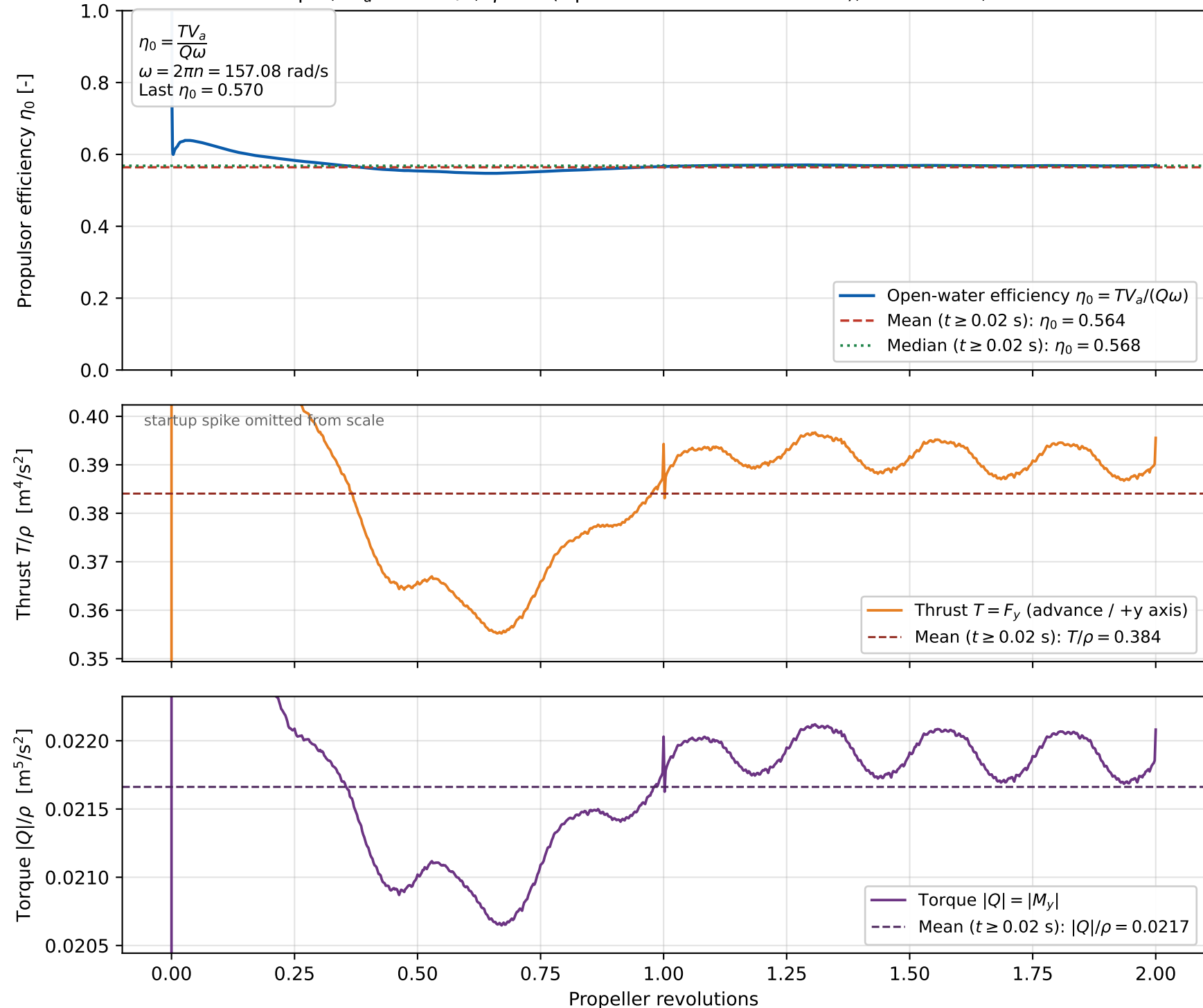
Propulsor efficiency — OpenFOAM propeller demo (coarse mesh) n = 1500 rpm, V_a = 5.0 m/s, \rho = 1 (OpenFOAM kinematic forces), \sim 86k cells, 2 revolutions
