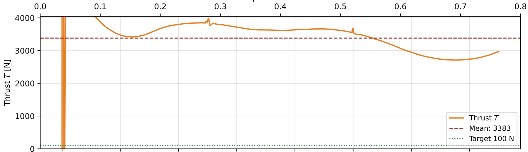
Thrust and torque vs time — n = 3200 rpm
