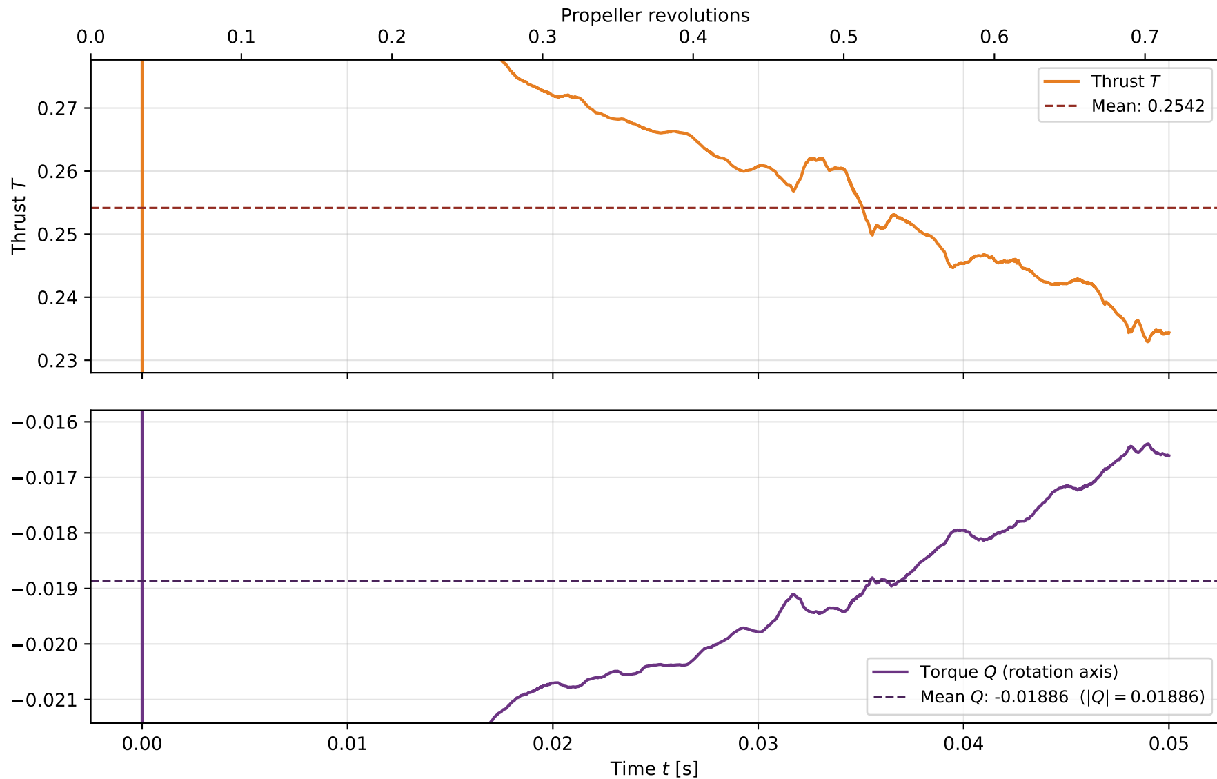
Thrust and torque vs time — n = 900 rpm
