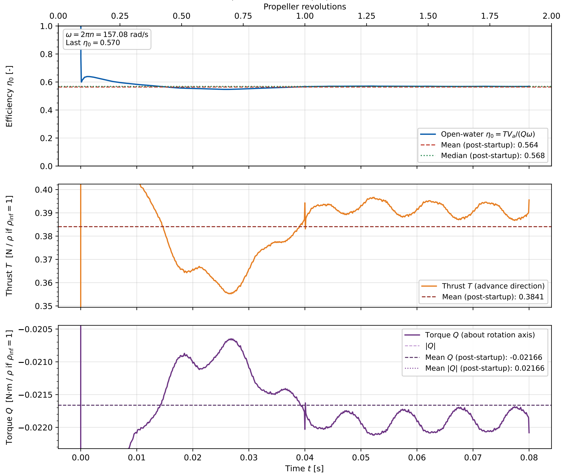
Propulsor performance vs time — n = 1500 rpm, |V_a| = 5.00 m/s OpenFOAM tutorial propeller (demo)
