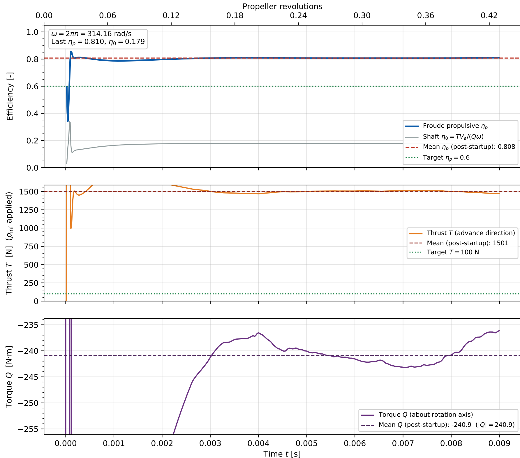
Propulsor performance vs time — n = 3000 rpm, |V_a| = 9.00 m/s v3 fix: meridional view, moderate load, \rho=1000 , 6-proc
