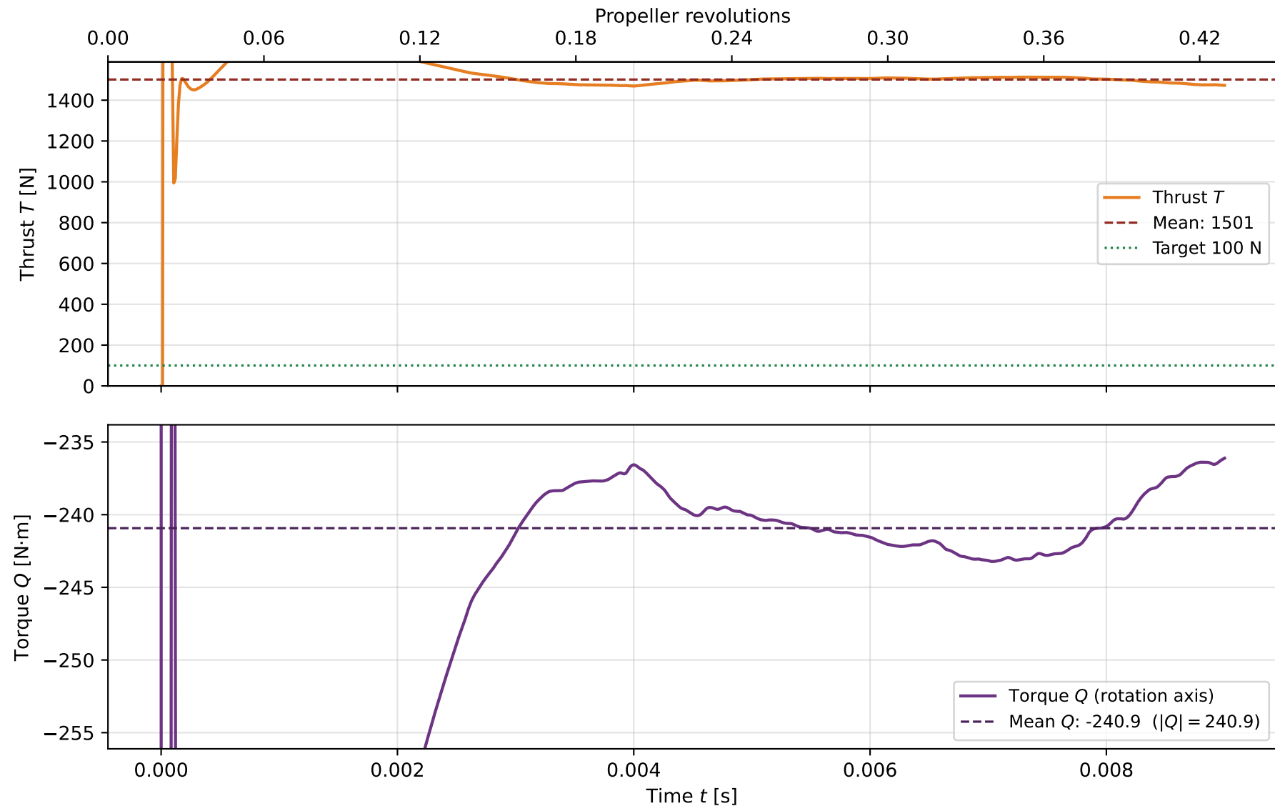
Thrust and torque vs time — n = 3000 rpm
