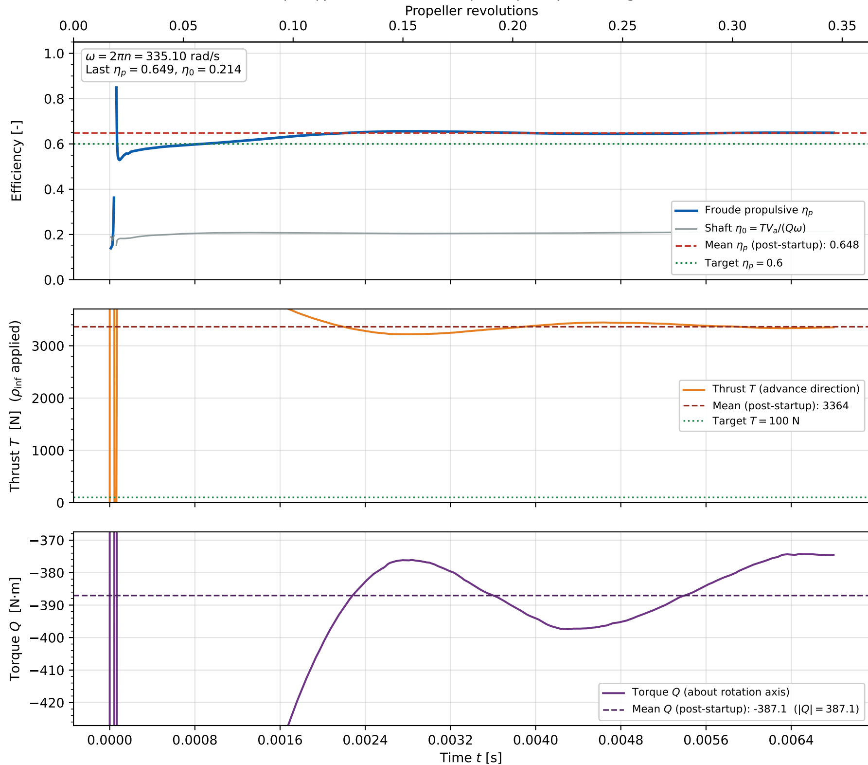
Propulsor performance vs time — n = 3200 rpm, |V_a| = 8.00 m/s pumpjet MRF v3 — 3200 rpm, 6-proc, \rho = 1000 kg/m 3
