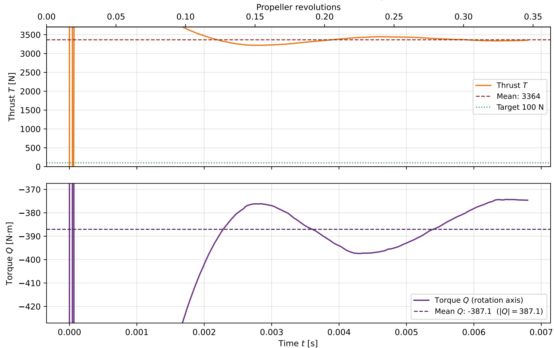
Thrust and torque vs time — n = 3200 rpm
