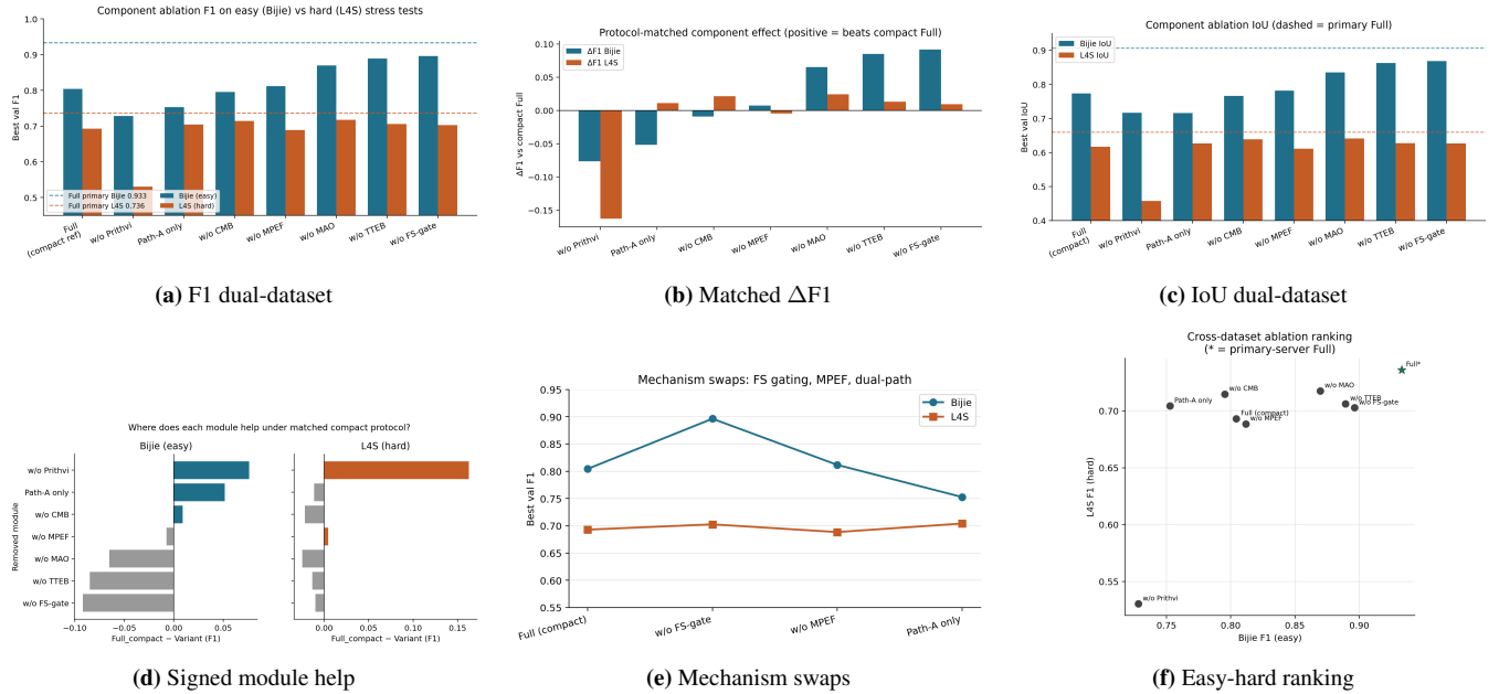
Figure 13: Comparative ablation panel. Dashed lines / star markers denote primary-server Full (Bijie 0.933, L4S 0.736).
