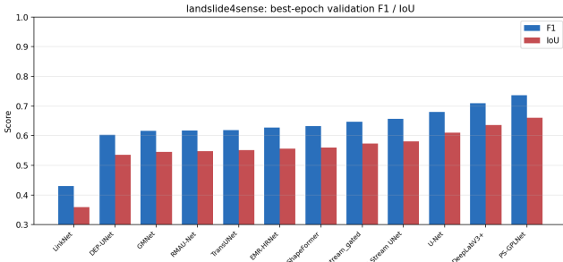
Figure 10: Landslide4Sense grouped best-epoch metrics including PS-GPLNet.
