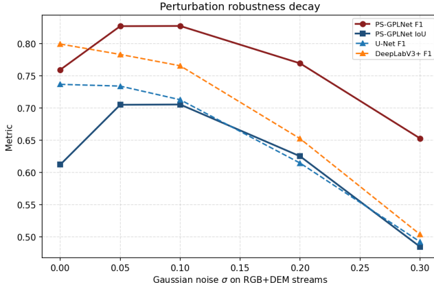
Figure 18: F1/IoU under RGB+DEM Gaussian noise. PS-GPLNet decays slower than U-Net and DeepLabV3+.
