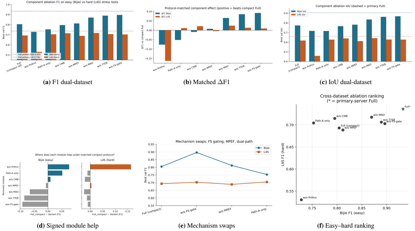
Figure 15: Comparative ablation panel. Dashed lines / star markers denote primary-server Full (Bijie 0.933, L4S 0.736).
