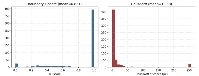
Figure 17: Boundary F-score and Hausdorff histograms on Bijie val predictions (PS-GPLNet).
