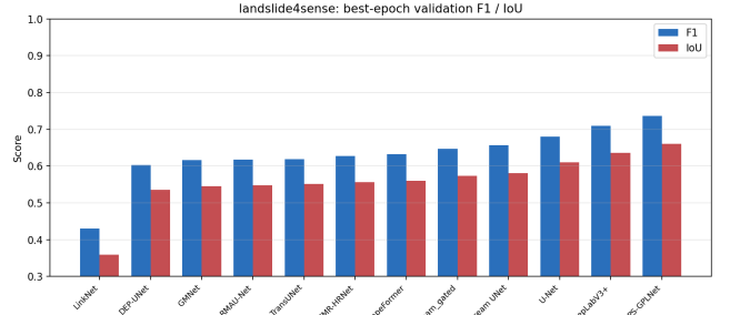
Figure 10: Landslide4Sense grouped best-epoch metrics including PS-GPLNet.
