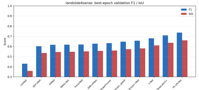
Figure 10: Landslide4Sense grouped best-epoch metrics including PS-GPLNet.
