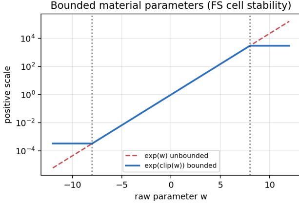
Figure 2: Bounded material map \exp(\text{clip}(w)) versus unbounded \exp(w) .
