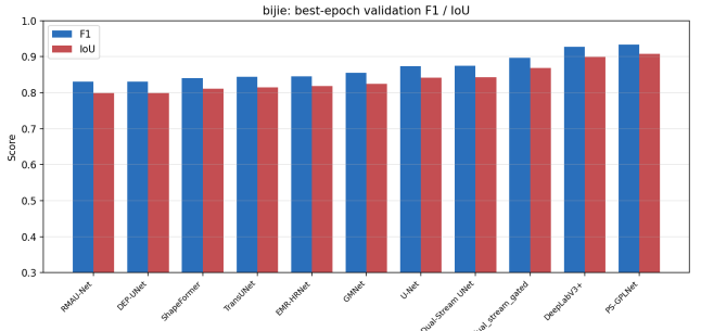
Figure 9: Bijie grouped best-epoch metrics including PS-GPLNet.
