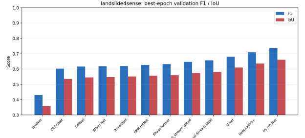
Figure 2: Landslide4Sense grouped metrics at each model’s best validation epoch.
