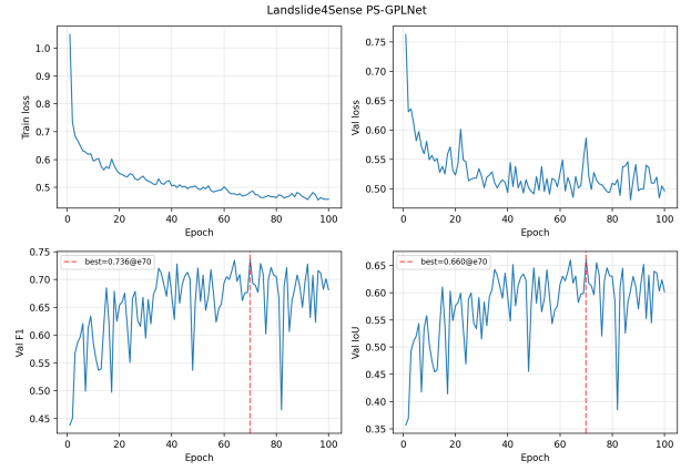
Figure 10: PS-GPLNet training dynamics on Landslide4Sense.
