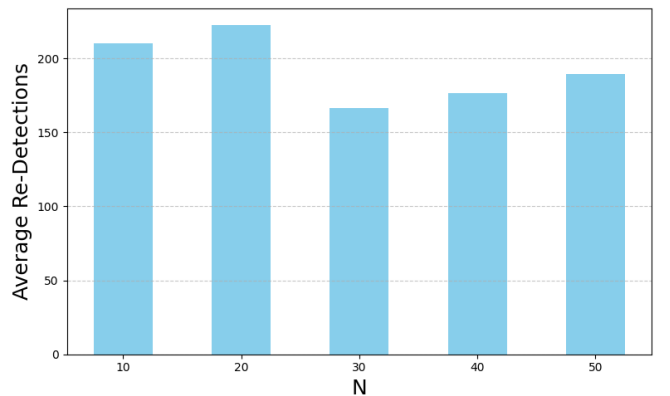
Figure 2. Average number of re-detection frames for different numbers of sample points
