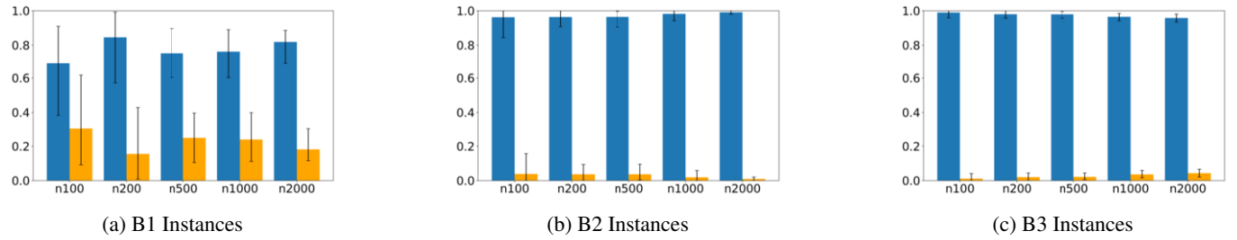
Figure 2: Average proportions of bin patterns in final solutions provided by the construction heuristic (blue bars) and by CG (yellow bars) for instance groups B1, B2, and B3.
