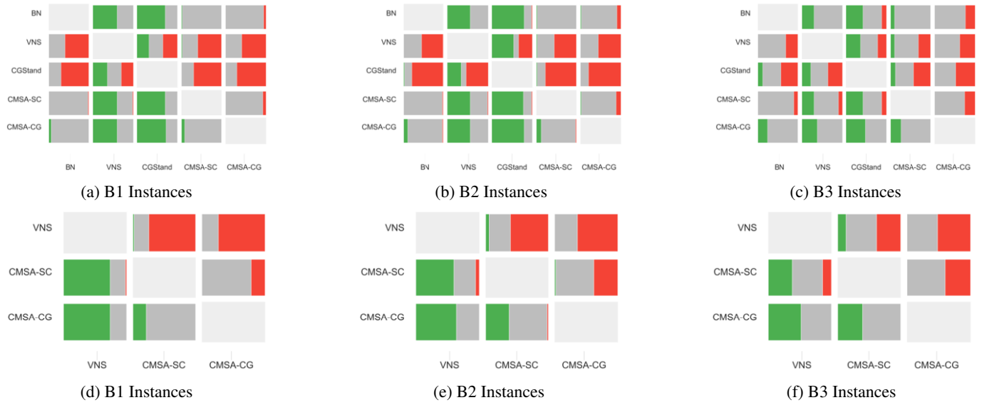
Figure 1: Pairwise stacked-bar advantage plots for best solutions (top row, panels a–c) and average solutions (bottom row, panels d–f) on instance classes B1, B2, and B3. Each cell reports how often the algorithm named by the row outperforms, ties, or is outperformed by the algorithm named by the column. Algorithm codes: BN=Best-Known, VNS=VNS, CGStand=CGStandalone, CMSA-SC=CMSA-SetCov, CMSA-CG=CMSA-ColGen.
