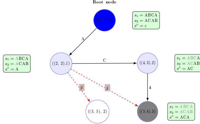
Fig. 1: \text{ROOTEDSUBSPACE}(u = ((1, 1), 0)) between \boxed{\text{A}}\text{BCA} and \boxed{\text{A}}\text{CAB} , assuming G_1 = G_2 = 1 . A final/terminal state is displayed in gray. The white-filled node is a valid LCS node, but not an VGLCS node—the second gap constraint is violated. The longest solution generated from this subspace is ACA .
