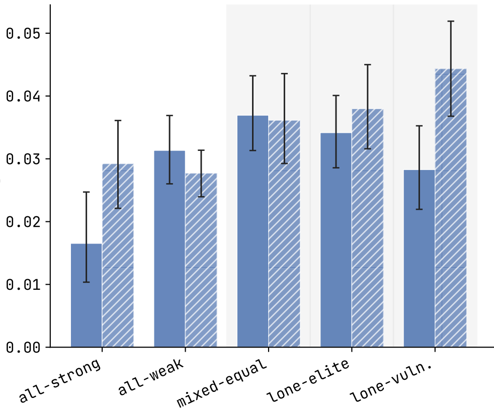
Gini coefficient of payoffs (mean of 20 games, 95% CI)
