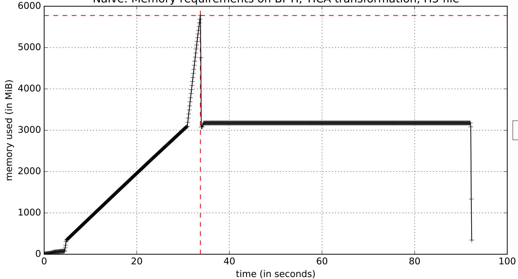
Naive: Memory requirements on BPTI, TICA transformation, H5 file
