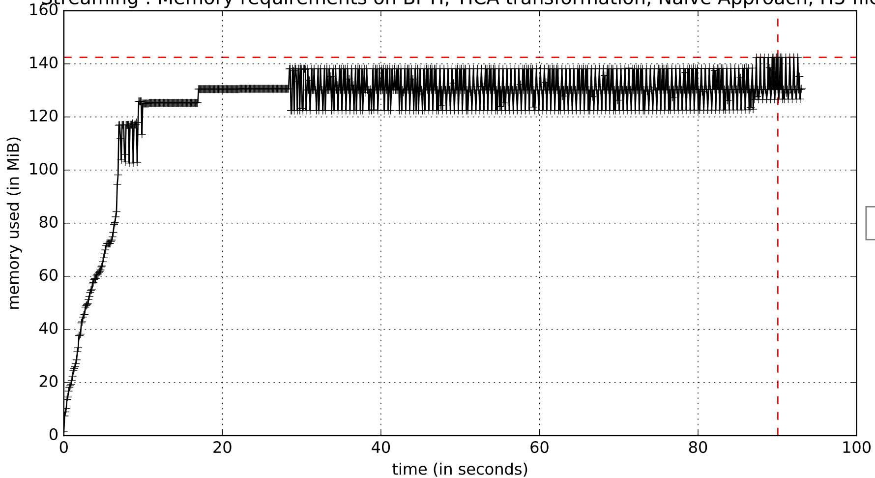
Streaming : Memory requirements on BPTI, TICA transformation, Naive Approach, H5 file
