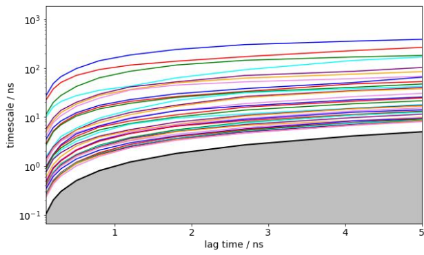
Implied time scale plot
