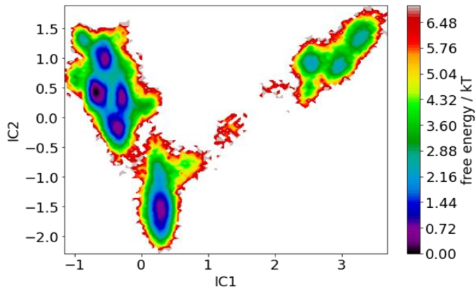
Free Energy Plot
