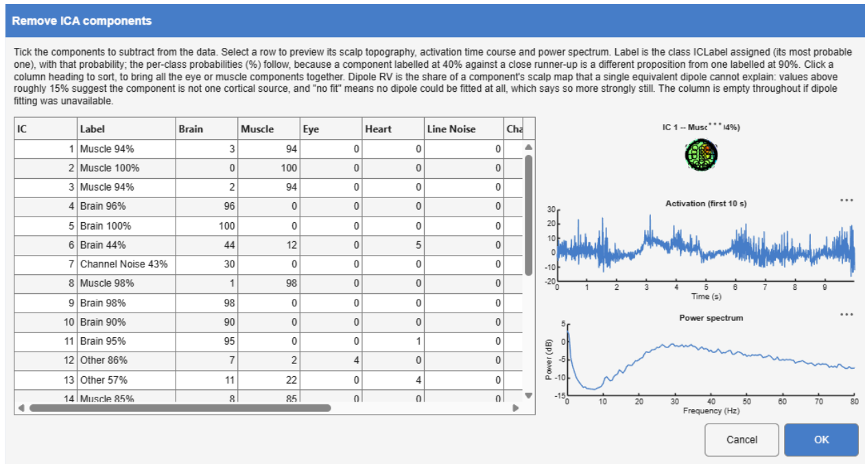
Figure 8.8: ICA on the ERP CORE MMN recording: each component's ICLabel class and probabilities, sortable by any column, and a preview of the selected component.
